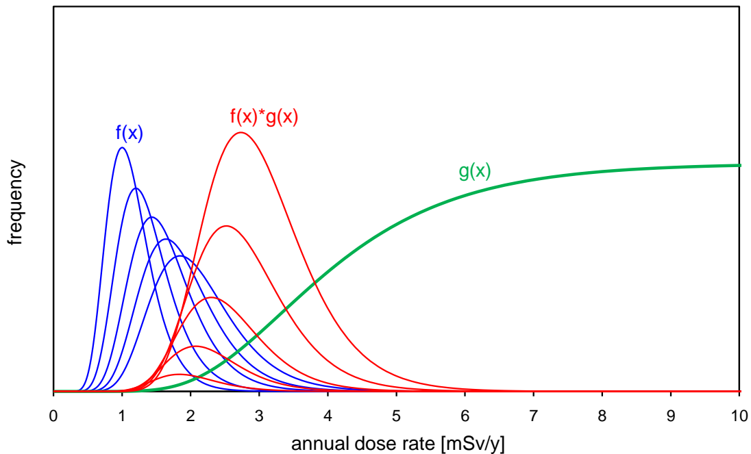
Figure A8: Frequency distribution for 5 values of the median dose rates (1.0, 1.2, 1.4, 1.6, 1.8 mSv/y, blue lines) und probability of a radiation damage (green line). The area below the red lines is proportional to the number of affected individuals.
